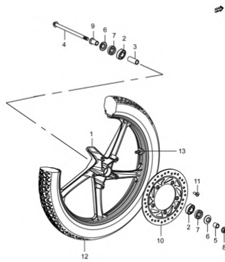
Fig. 42 FRONT WHEEL (P05-S410-0030)
