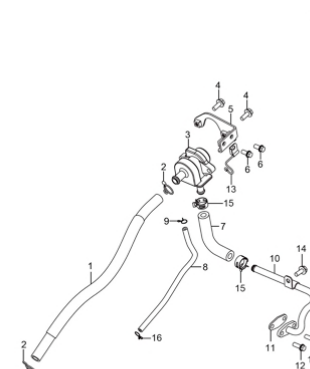
Fig. 12 2ND AIR VAVLE (P05-S120-0020)
