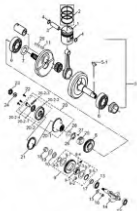
Fig. 5 CRANKSHAFT (P05-S050-0031)
