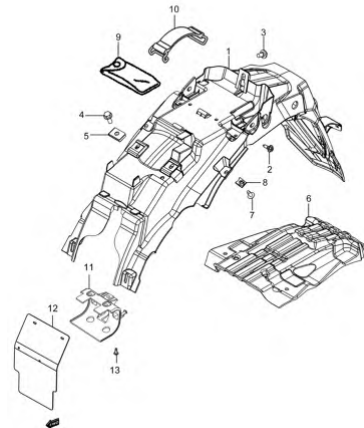
Fig. 40 COVER, SEAT TAIL (P05-S390-0032)
