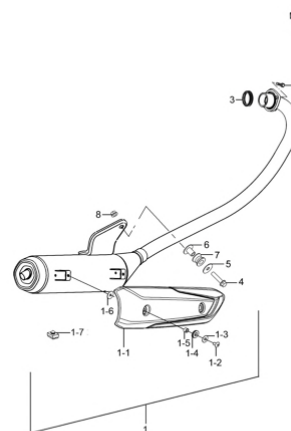
Fig. 11 MUFFLER (P05-S110-0036)
