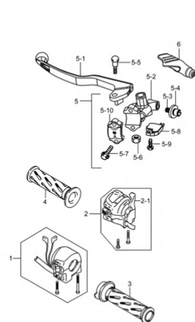
Fig. 35 HANDLE SWITCH (P05-S340-0037)
