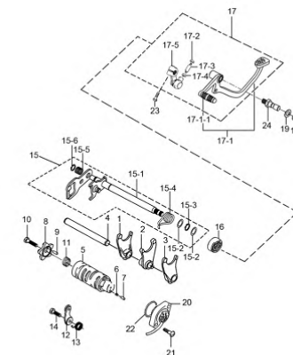
Fig. 16 GEAR SHIFTING (P05-S160-0018)
