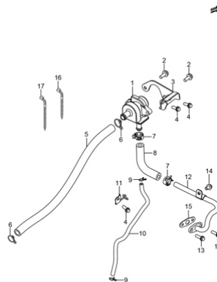
Fig. 11 2ND AIR VAVLE (P03-S120-0013)
