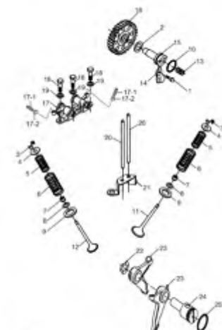
Fig. 7 CAMSHAFT-VALVE (P03-S070-0009)
