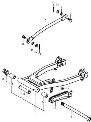
Fig. 41 REAR SWINGING ARM (P05-S440-0025)
