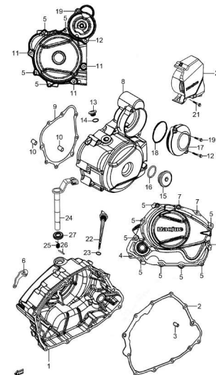
Fig. 4 CRANKCASE COVER (P05-S040-0048)
