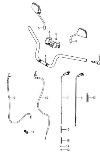
Fig. 32 HANDLEBAR (P05-S330-0069)
