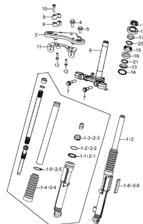
Fig. 39 STEERING STEM (P05-S400-0052)
