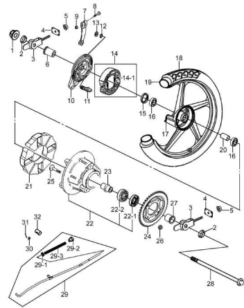
Fig. 43 REAR WHEEL (P05-S460-0075)
