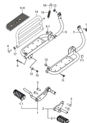
Fig. 28 FOOTREST (P05-S280-0045)
