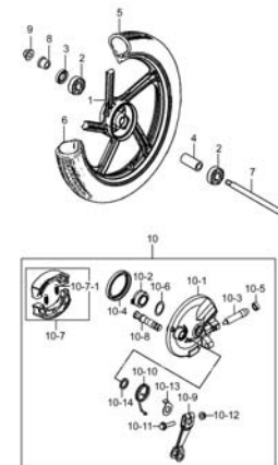
Fig. 40 FRONT WHEEL (X03-C410-0007)
