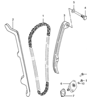
Fig. 8 CAM CHAIN (P07-S080-0008)
