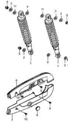
Fig. 44 REARSHOCK ABSORBER (P07-S450-0015)
