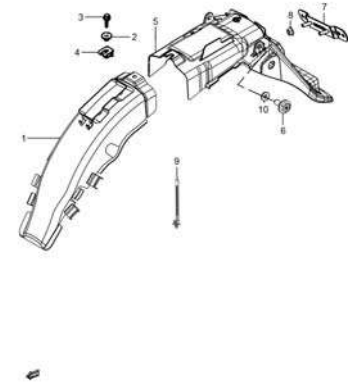
Fig. 40 COVER, SEAT TAIL (P07-S390-0022)
