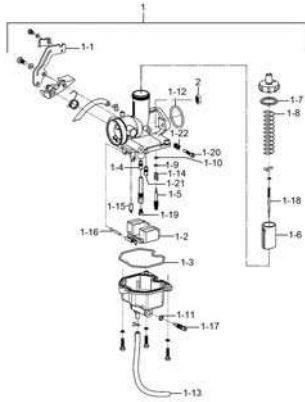
Fig. 9 CARBURETOR (P07-S090-0022)
