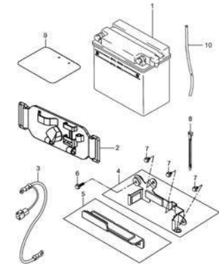
Fig. 20 BATTERY (P07-S190-0018)
