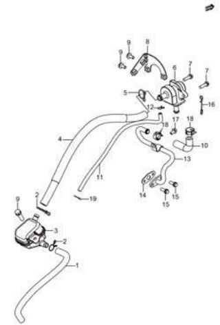
Fig. 12 2ND AIR VAVLE (P07-S120-0014)
