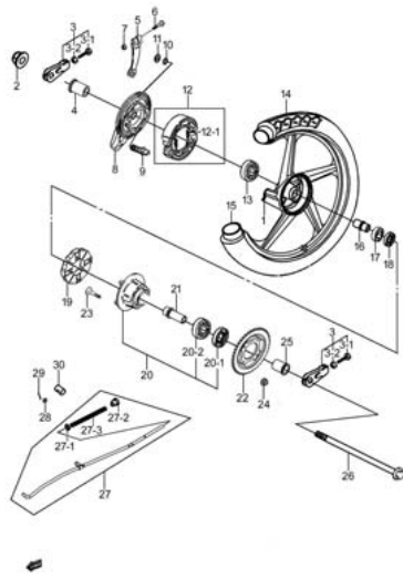
Fig. 42 REAR WHEEL (P10-S460-0001)
