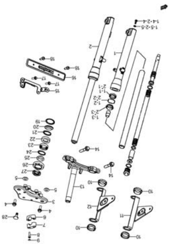
Fig. 38 STEERING STEM (P10-S400-0001)
