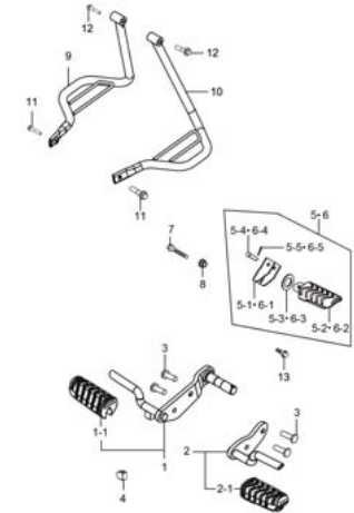
Fig. 28 FOOTREST (P10-S280-0001)
