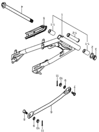
Fig. 40 REAR SWINGING ARM (P10-S440-0001)
