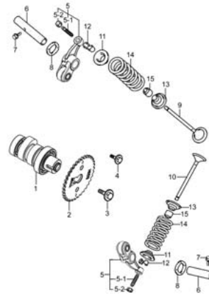
Fig. 7 CAMSHAFT-VALVE (P10-S070-0001)
