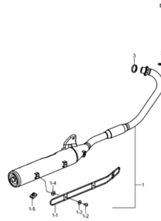
Fig. 11 MUFFLER (P10-S110-0001)
