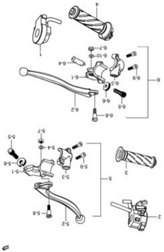
Fig. 34 HANDLE SWITCH (P10-S340-0001)
