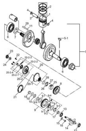
Fig. 5 CRANKSHAFT (P05-C050-0006)
