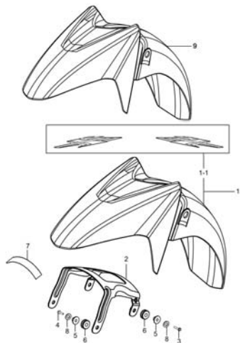
Fig. 33 FRONT FENDER (P05-C320-0003)
