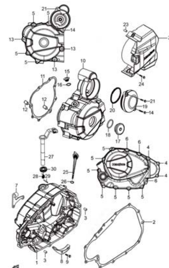
Fig. 4 CRANKCASE COVER (P05-C040-0001)
