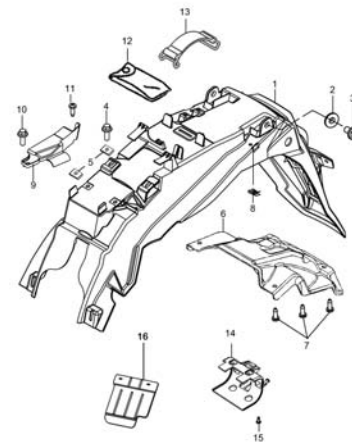
Fig. 36 REAR FENDER (P05-C350-0002)
